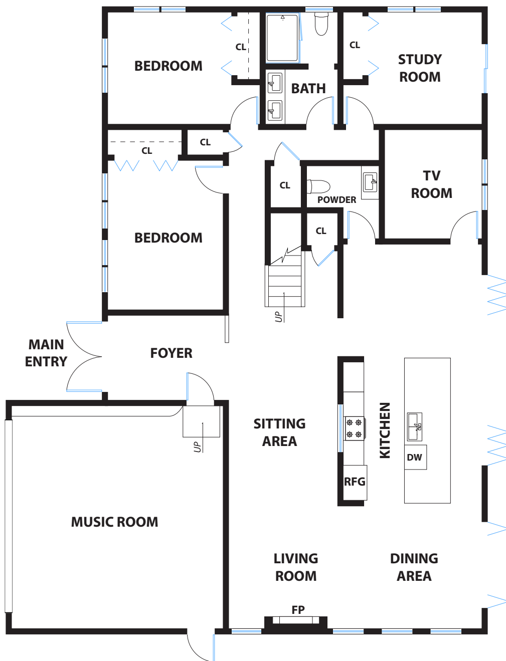
MAIN LEVEL
